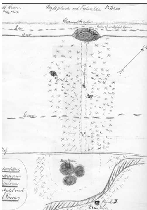
Situationsplan 1910
